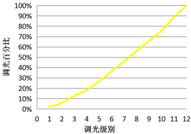
C-通道调光曲线 C channel Dimming Curve Graph
